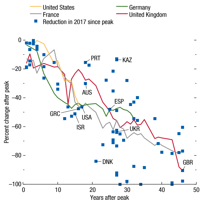
Figure 1.SF.10. Coal Phaseouts
